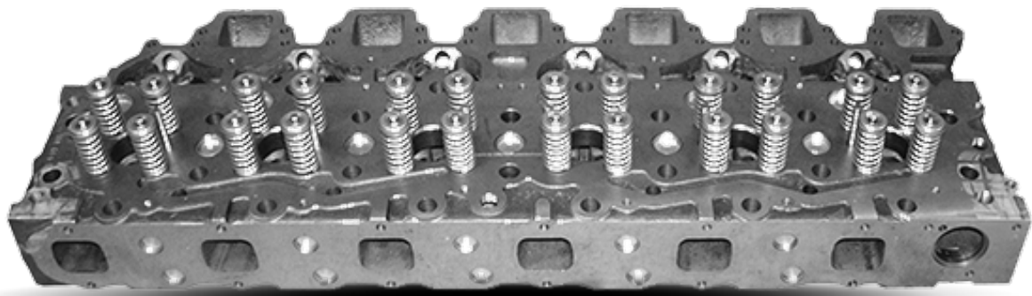
CYLINDER HEAD HEATED WITH VALVES
